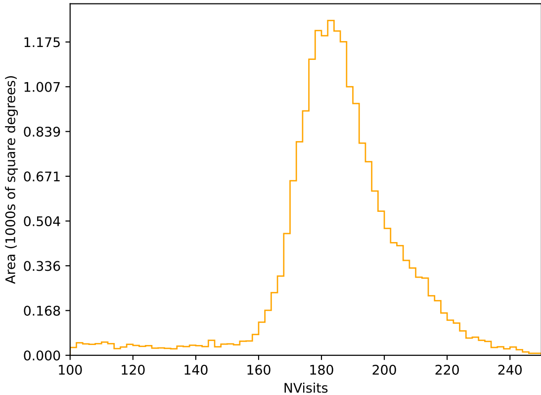
too_elab_r64_d3_griz_v3.4_10yrs All sky r band: NVisits
