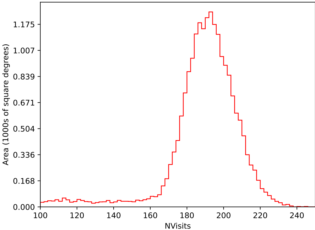
too_elab_r64_d3_griz_v3.4_10yrs All sky i band: NVisits
