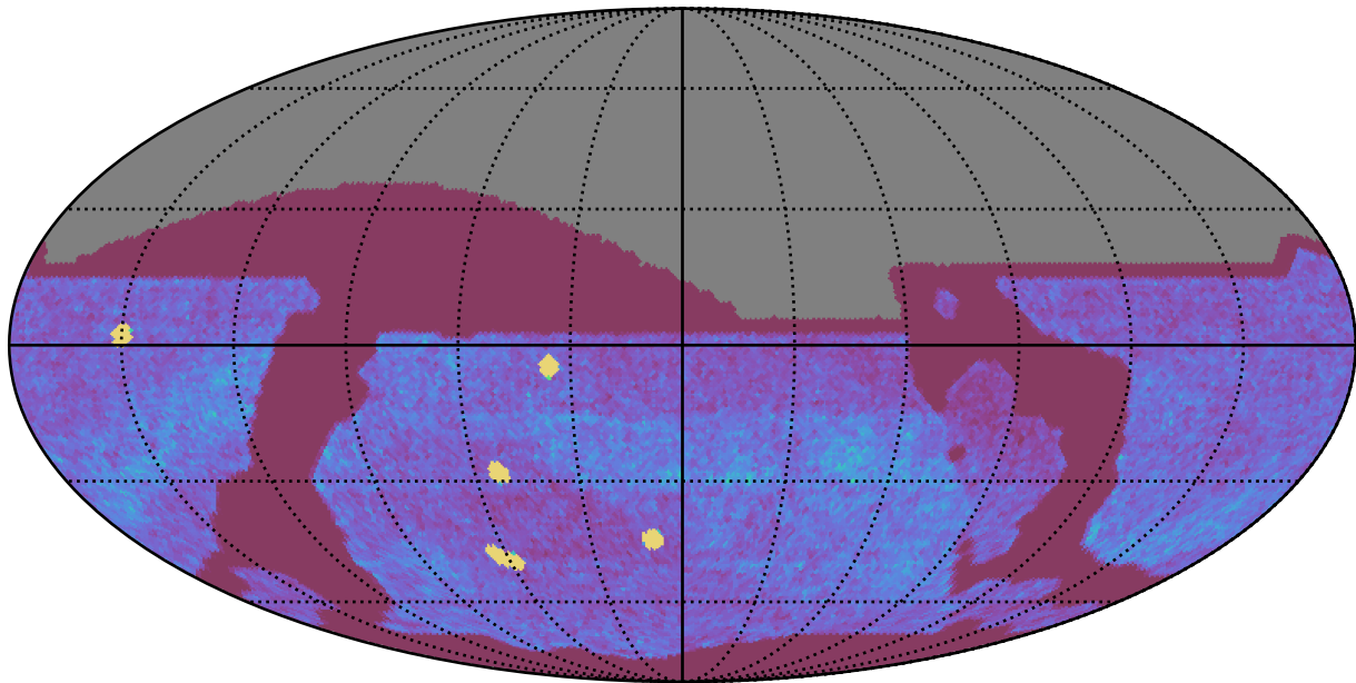
too_elab_r64_d3_griz_v3.4_10yrs All sky all bands: NVisits
