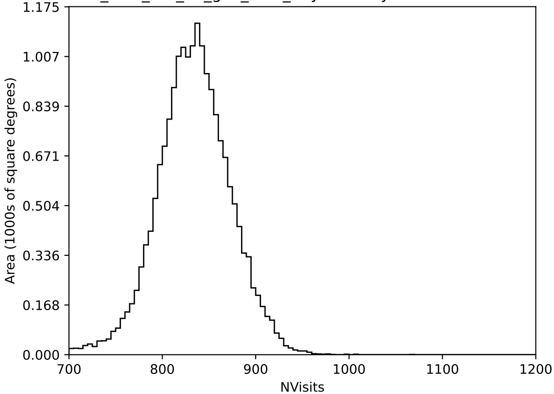
too_elab_r64_d3_griz_v3.4_10yrs All sky all bands: NVisits
