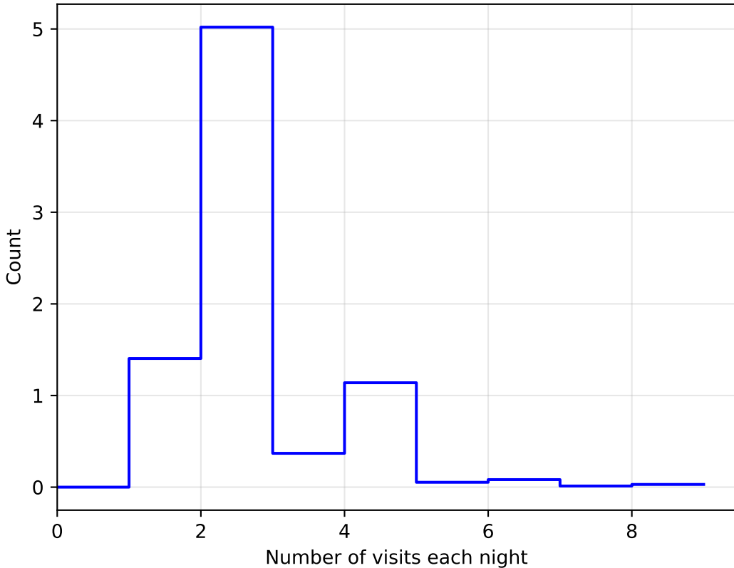
too_elab_r64_d3_griz_v3.4_10yrs WFD: NVisitsPerNight
