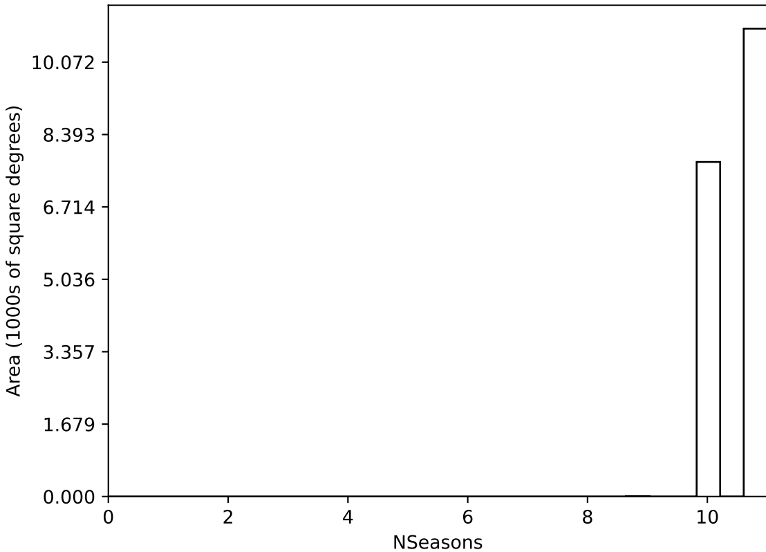
too_elab_r64_d3_griz_v3.4_10yrs WFD all bands: NSeasons
