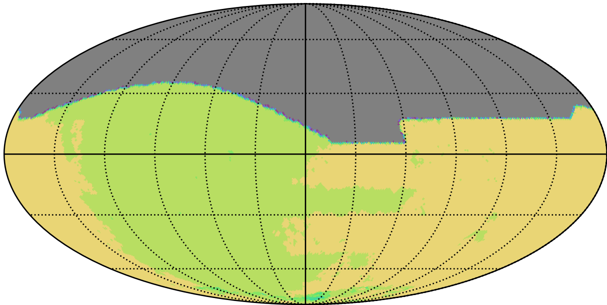
too_elab_r64_d3_griz_v3.4_10yrs All sky all bands: NSeasons
