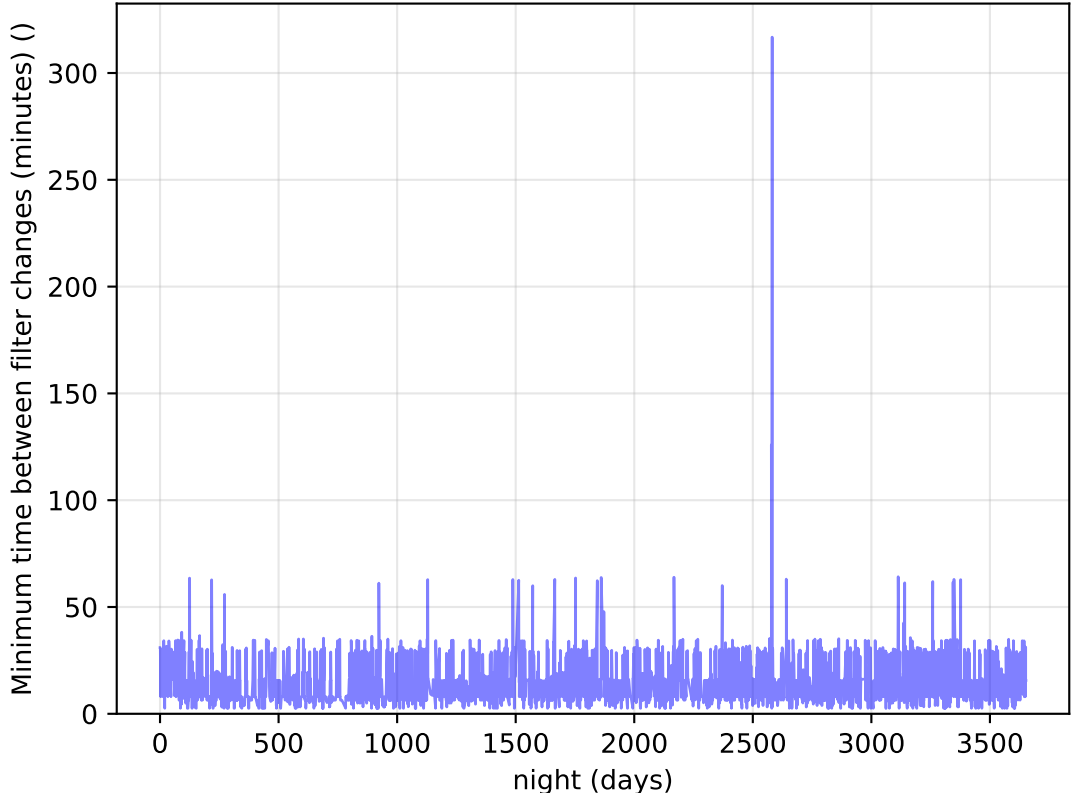
too_elab_r64_d3_griz_v3.4_10yrs Per Night: Minimum time between filter changes (minutes)
