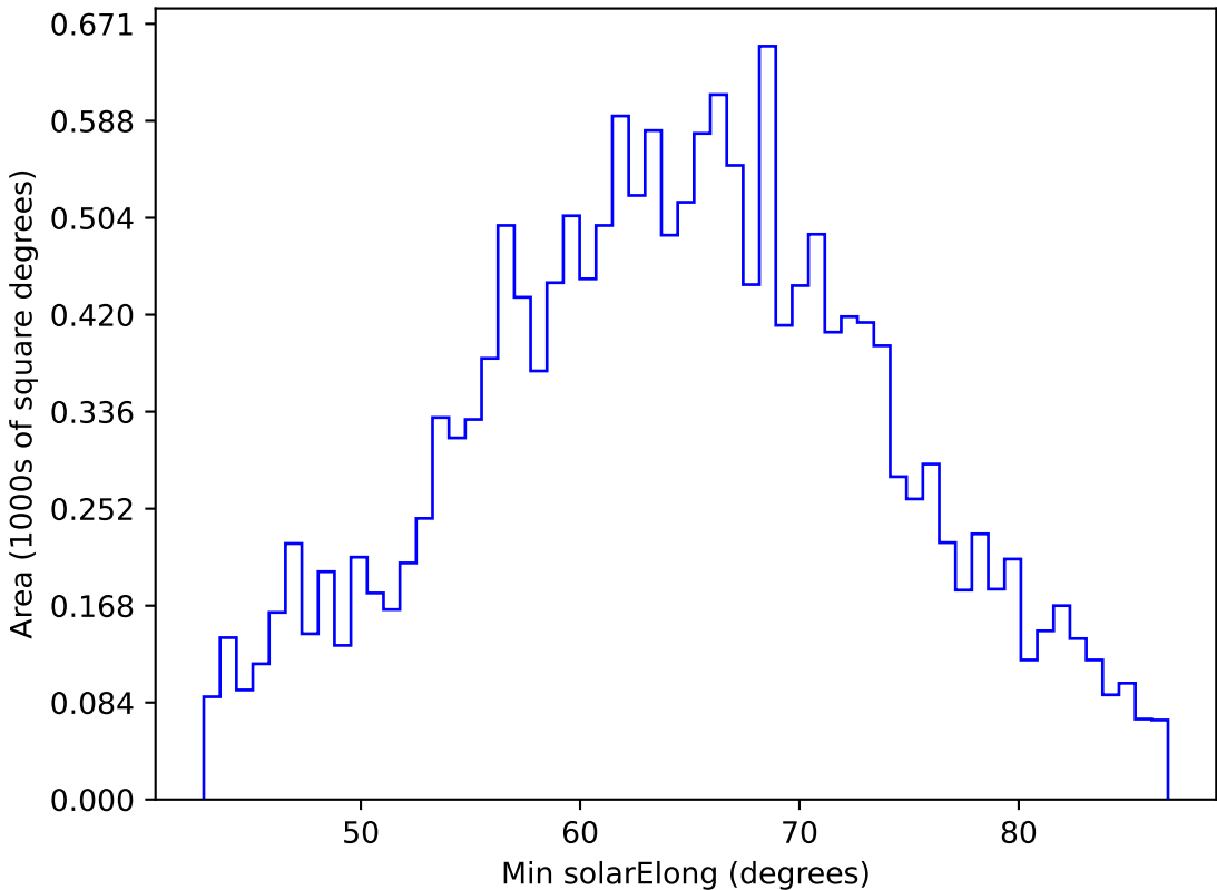
too_elab_r64_d3_griz_v3.4_10yrs WFD y band: Min solarElong
