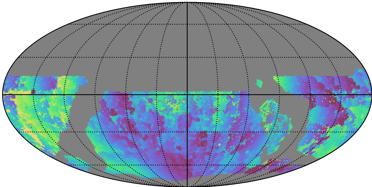
too_elab_r64_d3_griz_v3.4_10yrs WFD u band: Min solarElong
