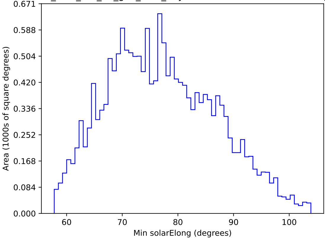
too_elab_r64_d3_griz_v3.4_10yrs WFD u band: Min solarElong
