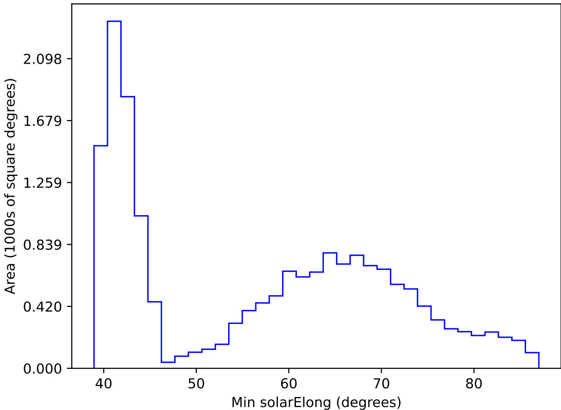
too_elab_r64_d3_griz_v3.4_10yrs WFD r band: Min solarElong
