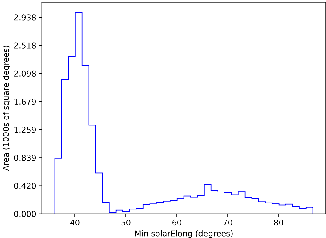
too_elab_r64_d3_griz_v3.4_10yrs WFD i band: Min solarElong
