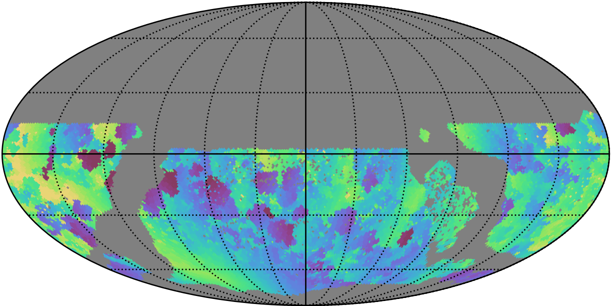
too_elab_r64_d3_griz_v3.4_10yrs WFD g band: Min solarElong
