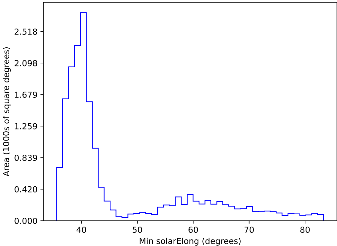
too_elab_r64_d3_griz_v3.4_10yrs WFD all bands: Min solarElong
