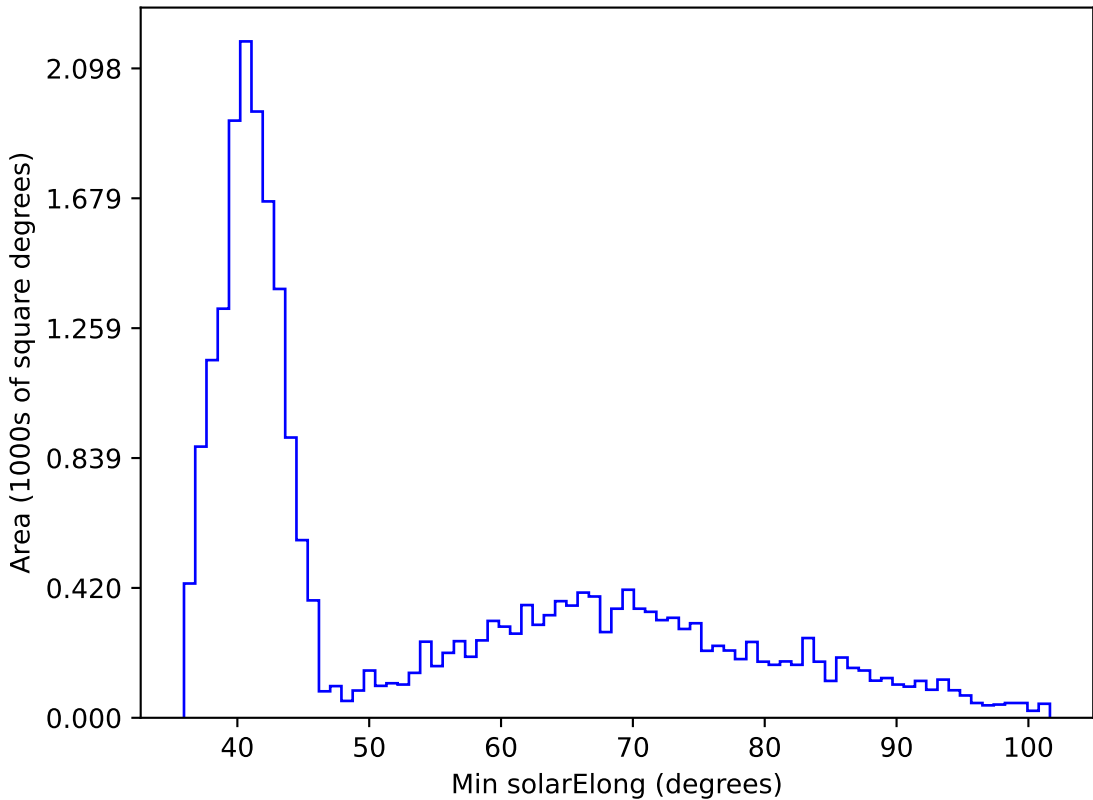
too_elab_r64_d3_griz_v3.4_10yrs All sky z band: Min solarElong
