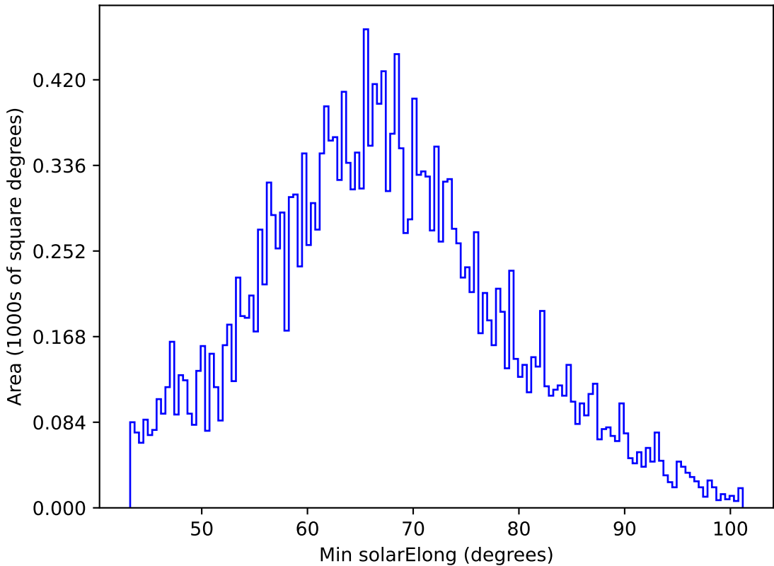
too_elab_r64_d3_griz_v3.4_10yrs All sky y band: Min solarElong
