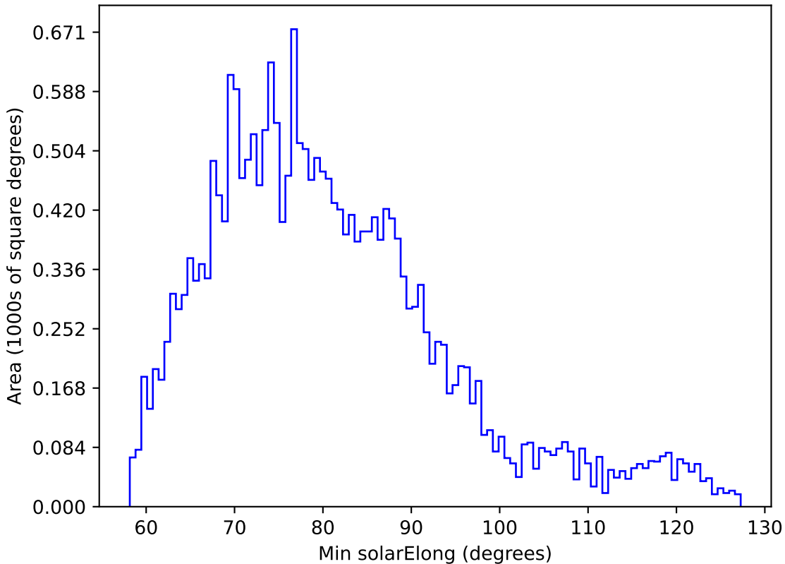
too_elab_r64_d3_griz_v3.4_10yrs All sky u band: Min solarElong
