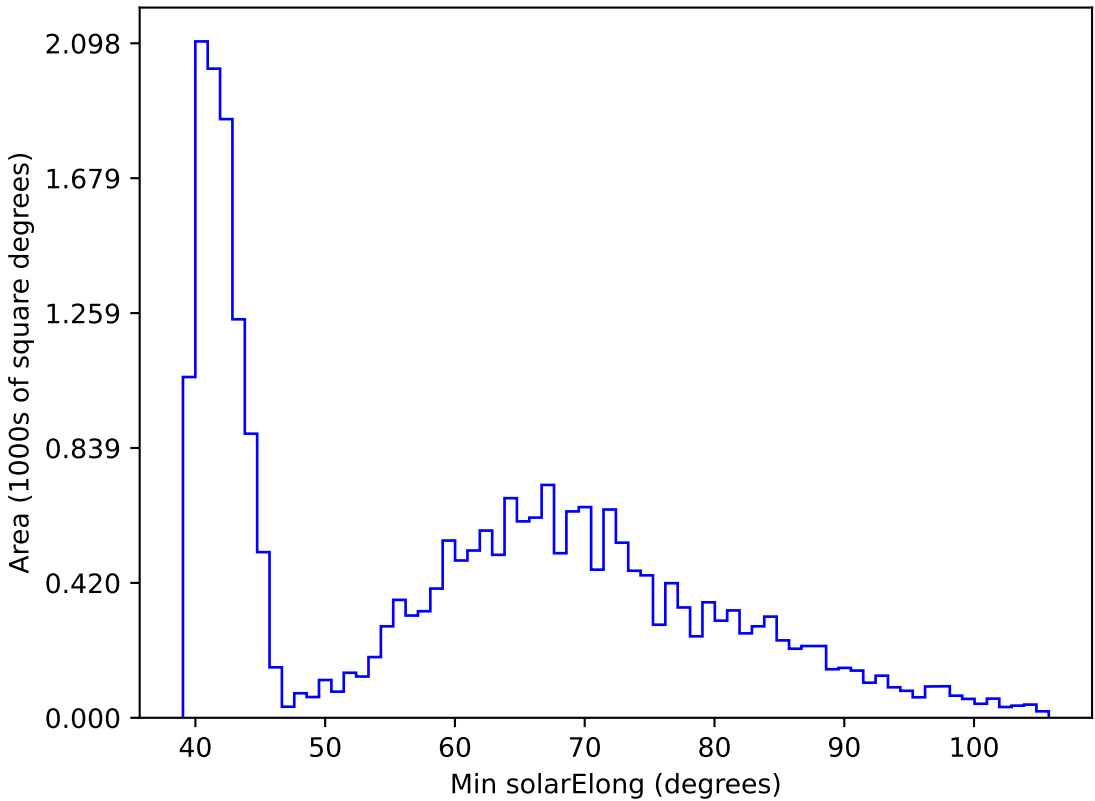
too_elab_r64_d3_griz_v3.4_10yrs All sky r band: Min solarElong
