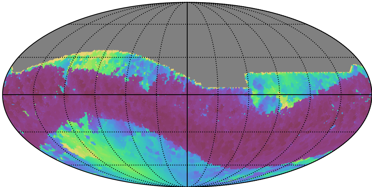
too_elab_r64_d3_griz_v3.4_10yrs All sky i band: Min solarElong
