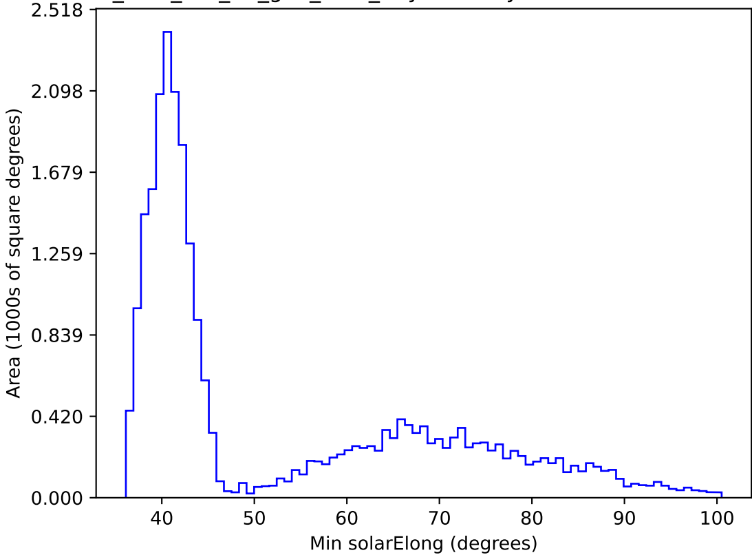
too_elab_r64_d3_griz_v3.4_10yrs All sky i band: Min solarElong
