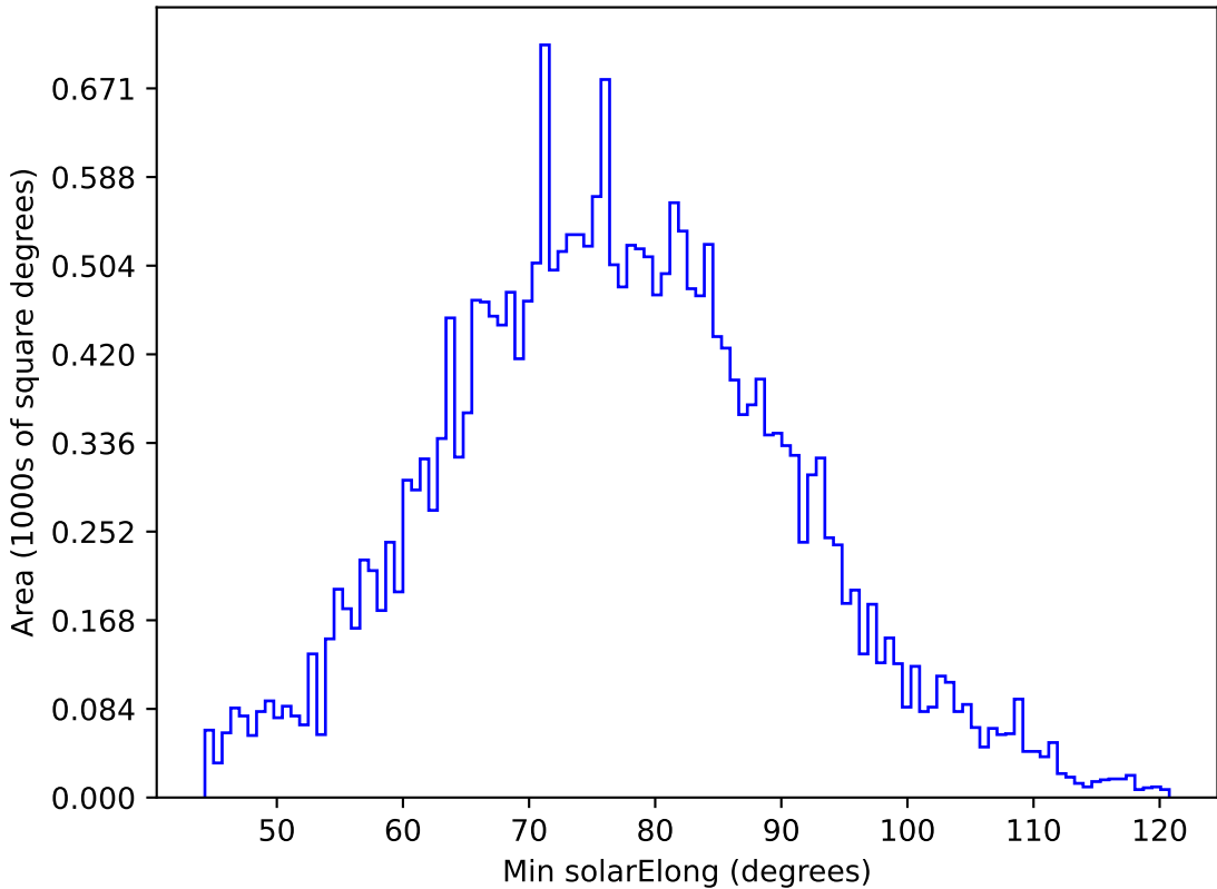
too_elab_r64_d3_griz_v3.4_10yrs All sky g band: Min solarElong
