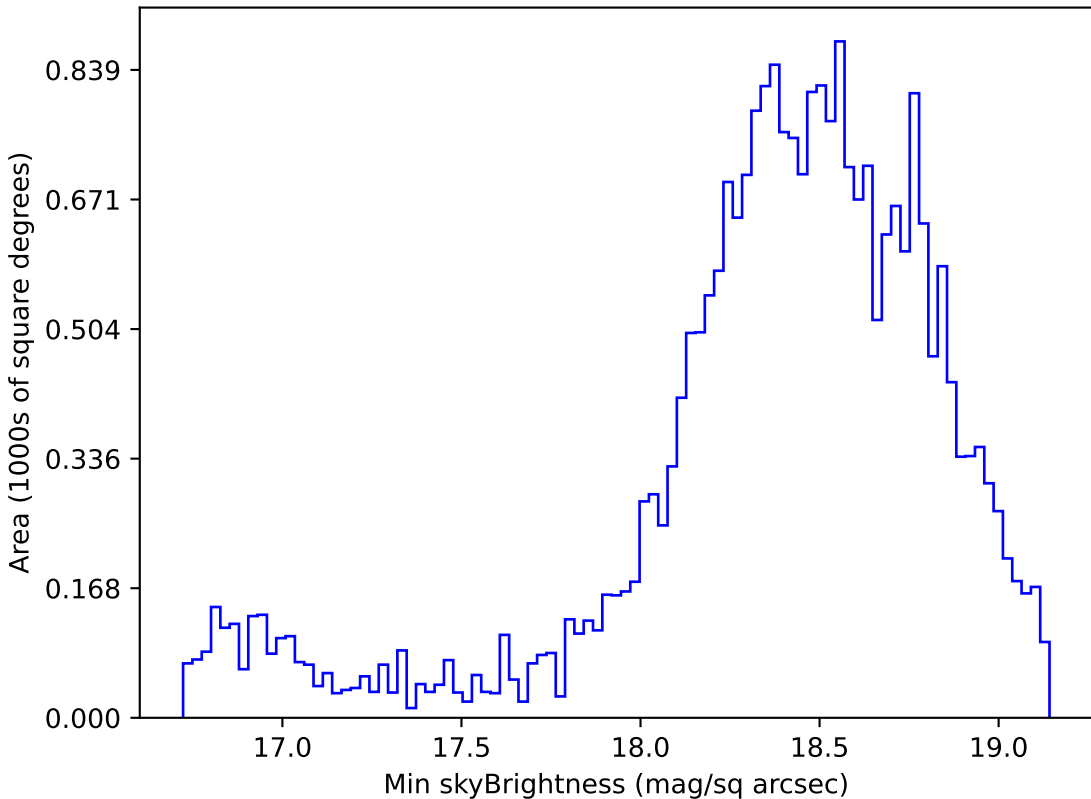
too_elab_r64_d3_griz_v3.4_10yrs Yr 1 z band: Min skyBrightness
