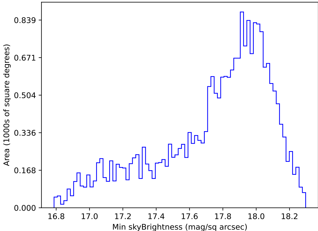
too_elab_r64_d3_griz_v3.4_10yrs Yr 1 y band: Min skyBrightness
