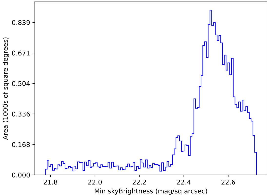
too_elab_r64_d3_griz_v3.4_10yrs Yr 1 u band: Min skyBrightness
