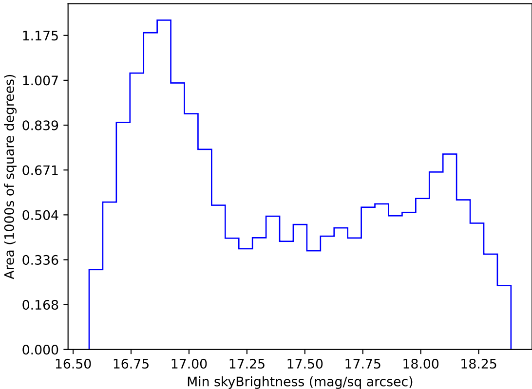
too_elab_r64_d3_griz_v3.4_10yrs WFD z band: Min skyBrightness
