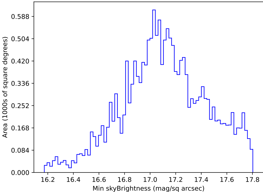
too_elab_r64_d3_griz_v3.4_10yrs WFD y band: Min skyBrightness
