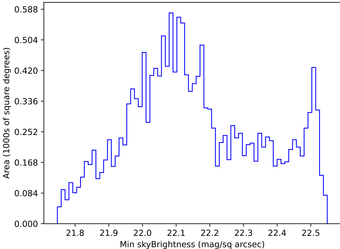
too_elab_r64_d3_griz_v3.4_10yrs WFD u band: Min skyBrightness
