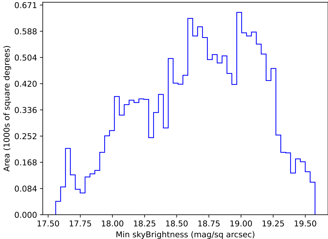
too_elab_r64_d3_griz_v3.4_10yrs WFD r band: Min skyBrightness
