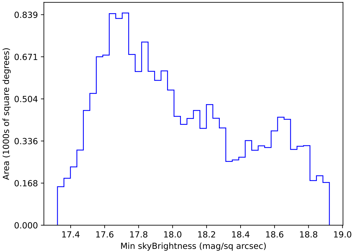
too_elab_r64_d3_griz_v3.4_10yrs WFD i band: Min skyBrightness
