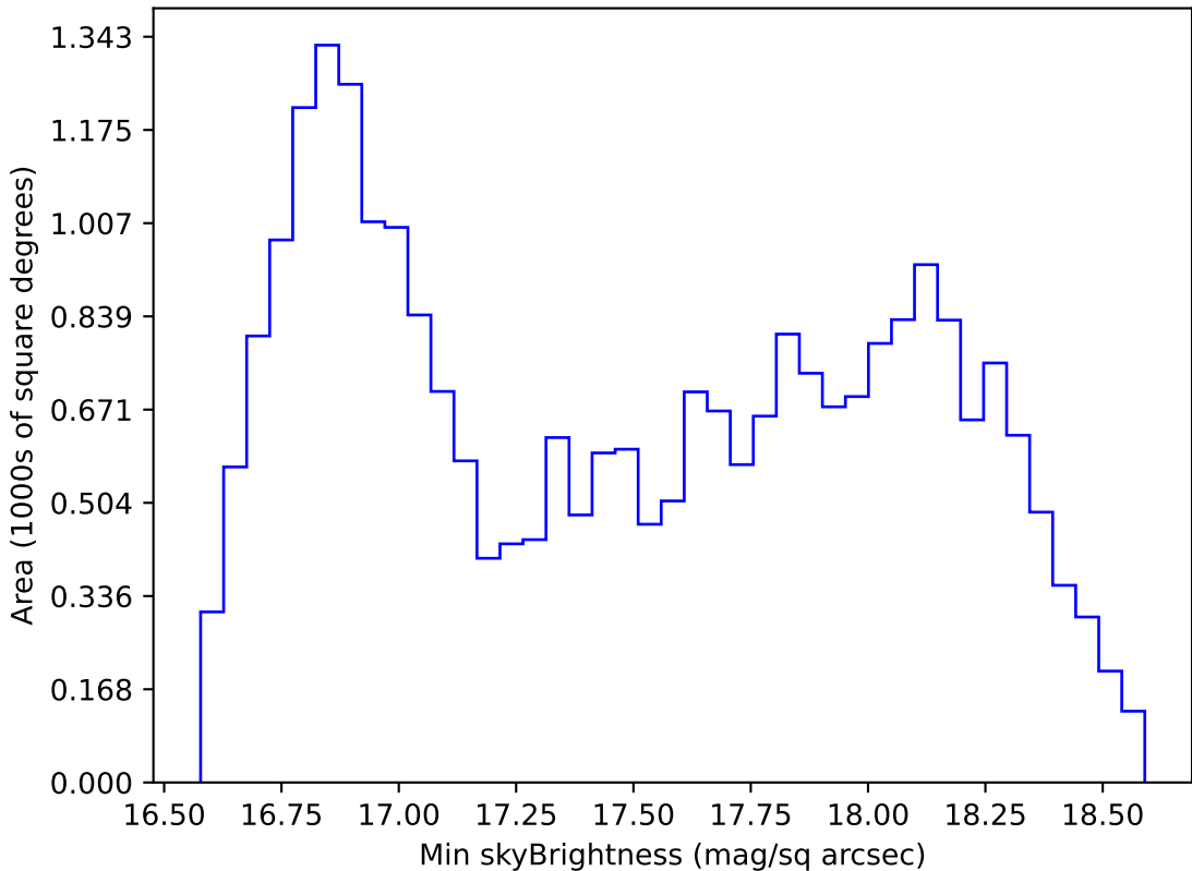
too_elab_r64_d3_griz_v3.4_10yrs All sky z band: Min skyBrightness
