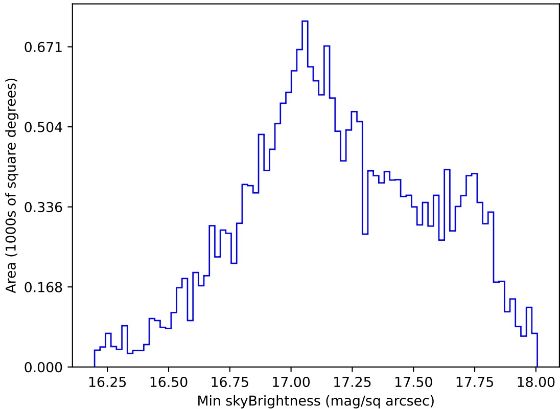
too_elab_r64_d3_griz_v3.4_10yrs All sky y band: Min skyBrightness
