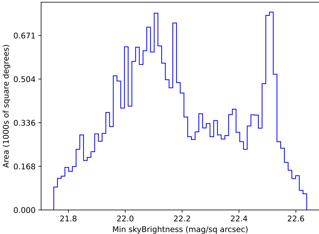
too_elab_r64_d3_griz_v3.4_10yrs All sky u band: Min skyBrightness
