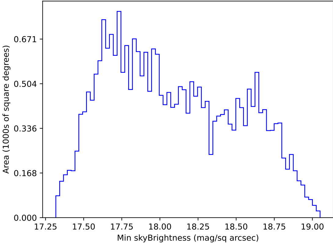
too_elab_r64_d3_griz_v3.4_10yrs All sky i band: Min skyBrightness
