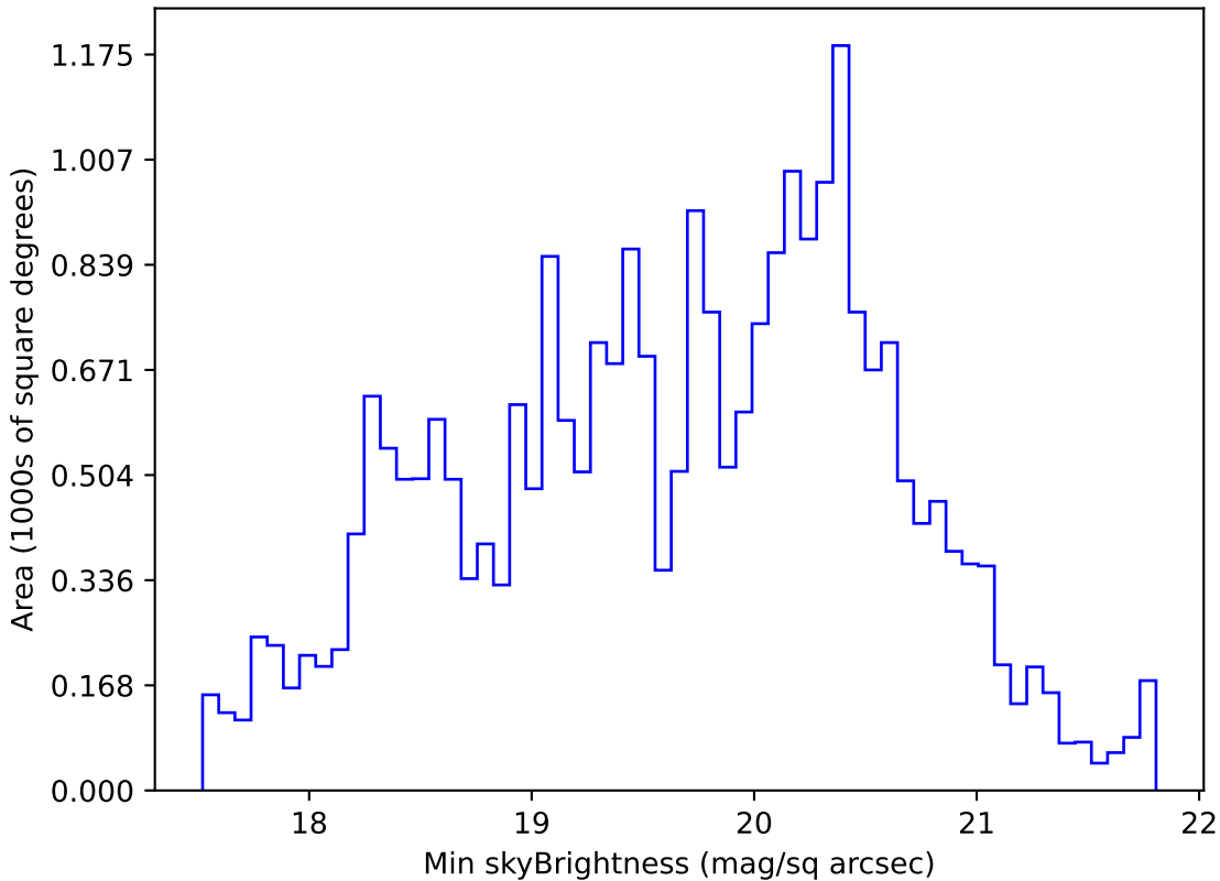
too_elab_r64_d3_griz_v3.4_10yrs All sky g band: Min skyBrightness
