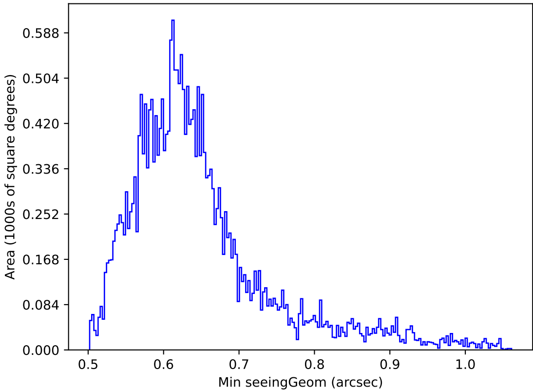
too_elab_r64_d3_griz_v3.4_10yrs Yr 1 z band: Min seeingGeom
