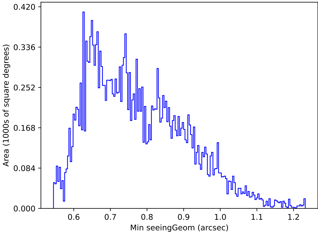
too_elab_r64_d3_griz_v3.4_10yrs Yr 1 u band: Min seeingGeom
