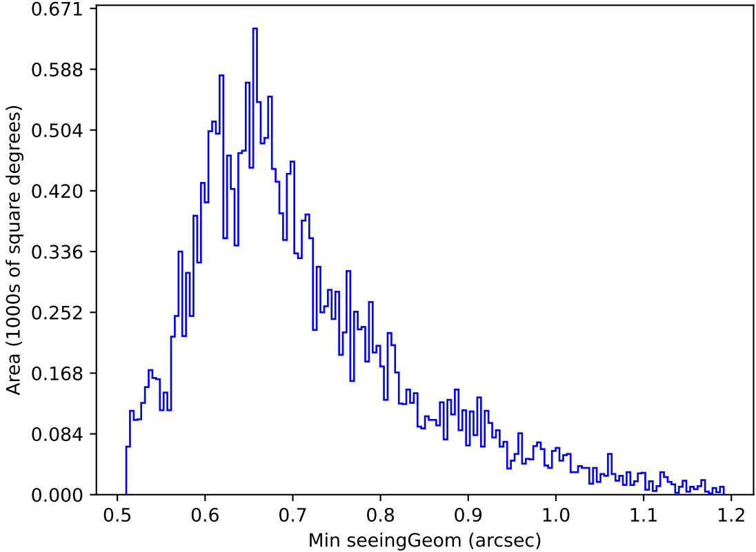
too_elab_r64_d3_griz_v3.4_10yrs Yr 1 g band: Min seeingGeom
