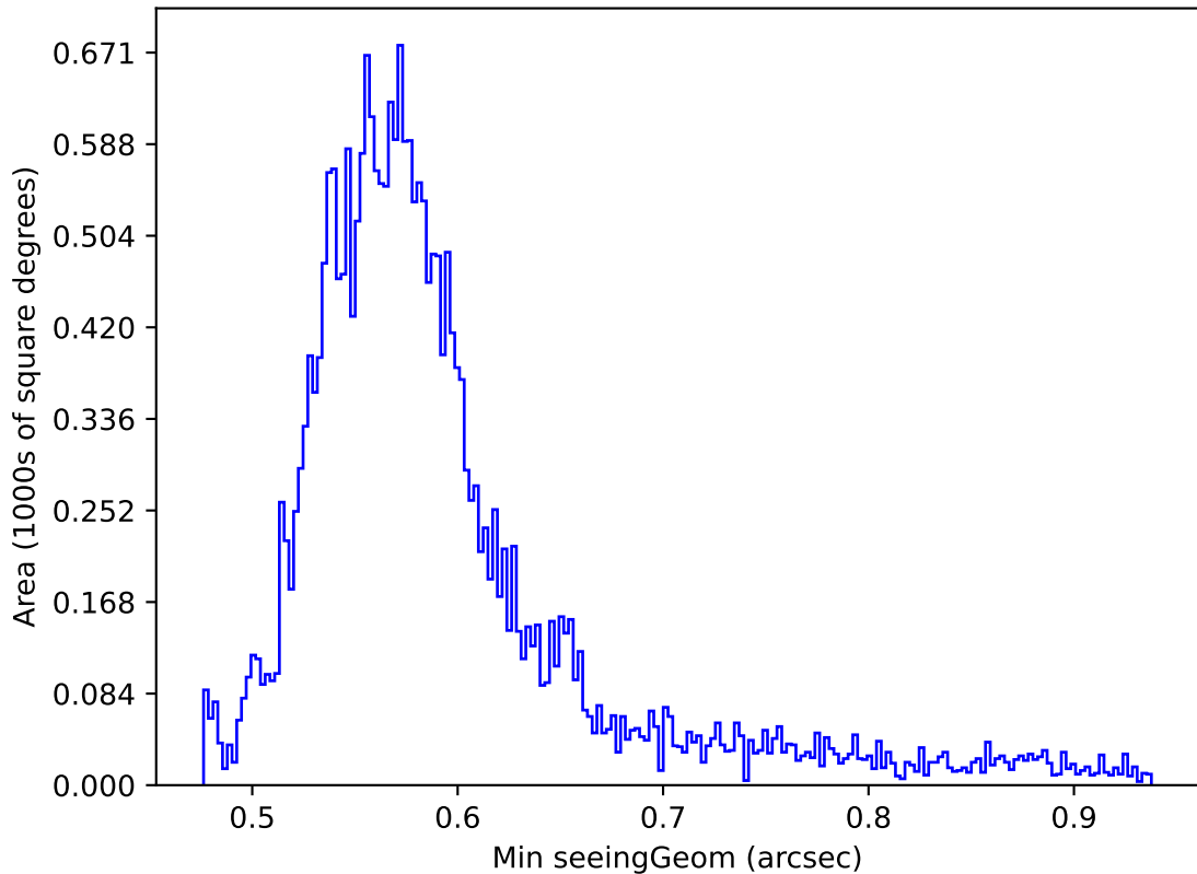
too_elab_r64_d3_griz_v3.4_10yrs Yr 1 all bands: Min seeingGeom
