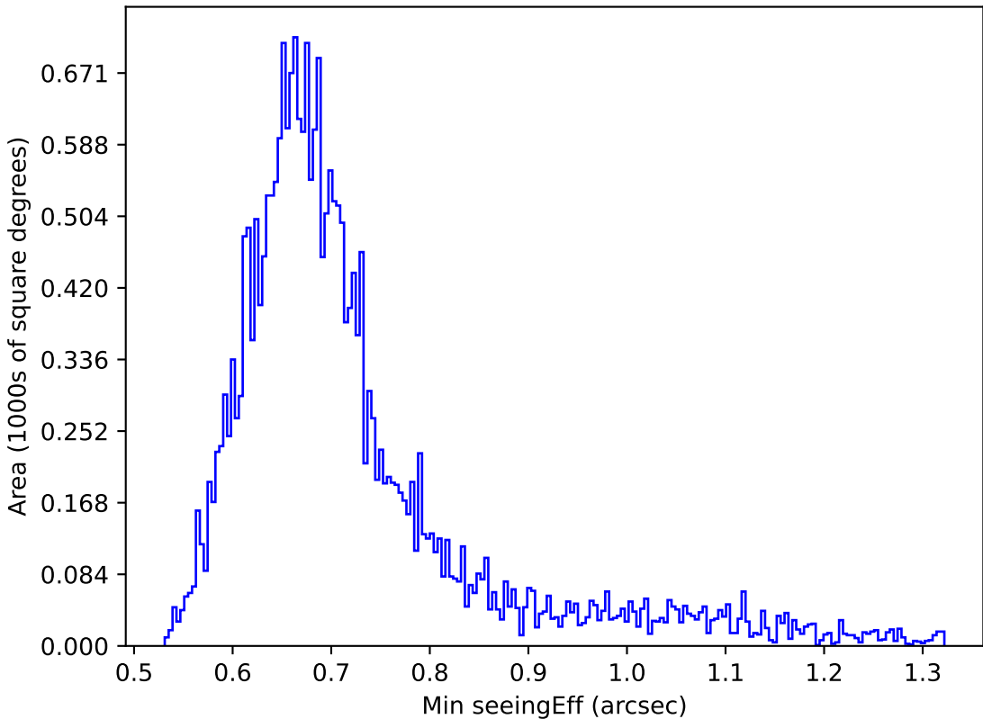
too_elab_r64_d3_griz_v3.4_10yrs Yr 1 r band: Min seeingEff
