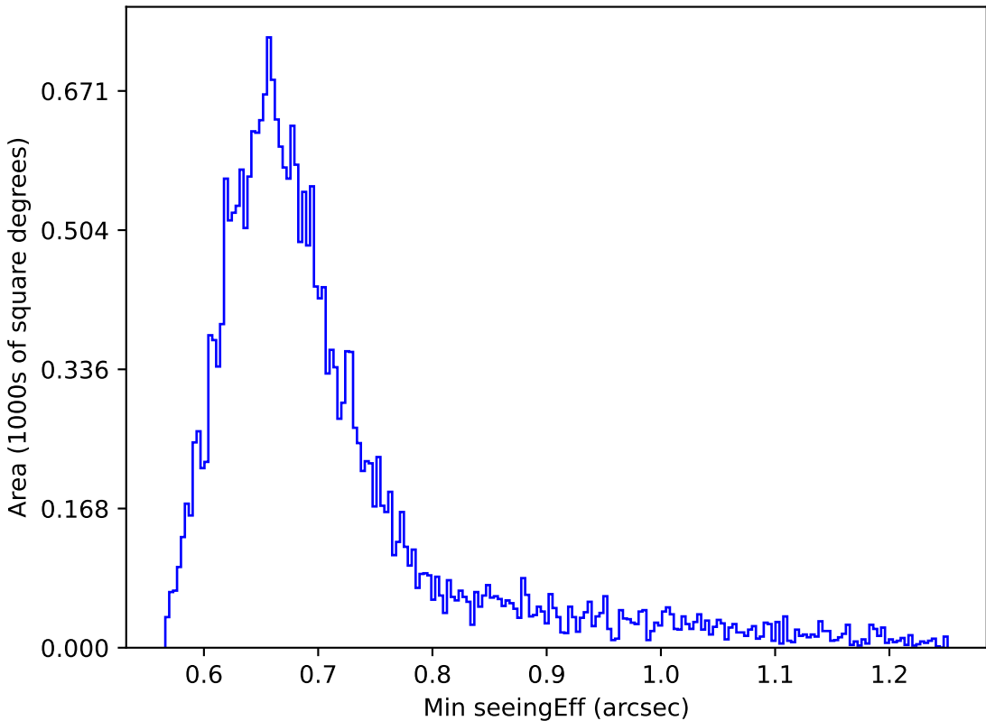
too_elab_r64_d3_griz_v3.4_10yrs Yr 1 i band: Min seeingEff
