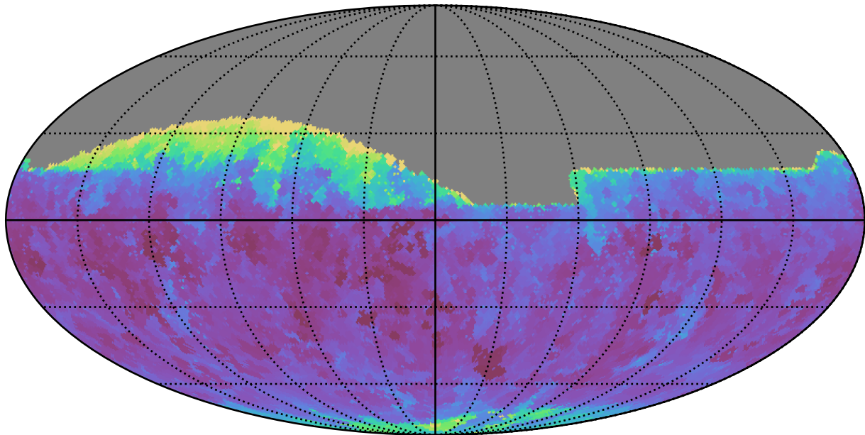
too_elab_r64_d3_griz_v3.4_10yrs Yr 1 all bands: Min seeingEff
