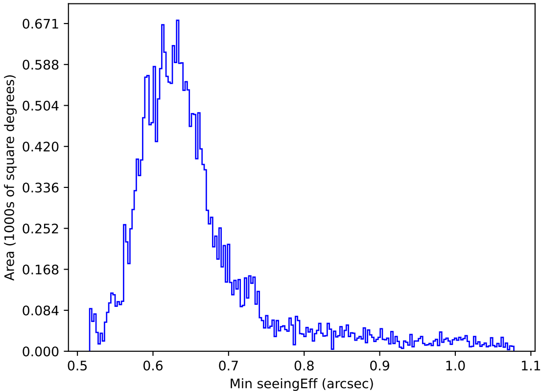
too_elab_r64_d3_griz_v3.4_10yrs Yr 1 all bands: Min seeingEff
