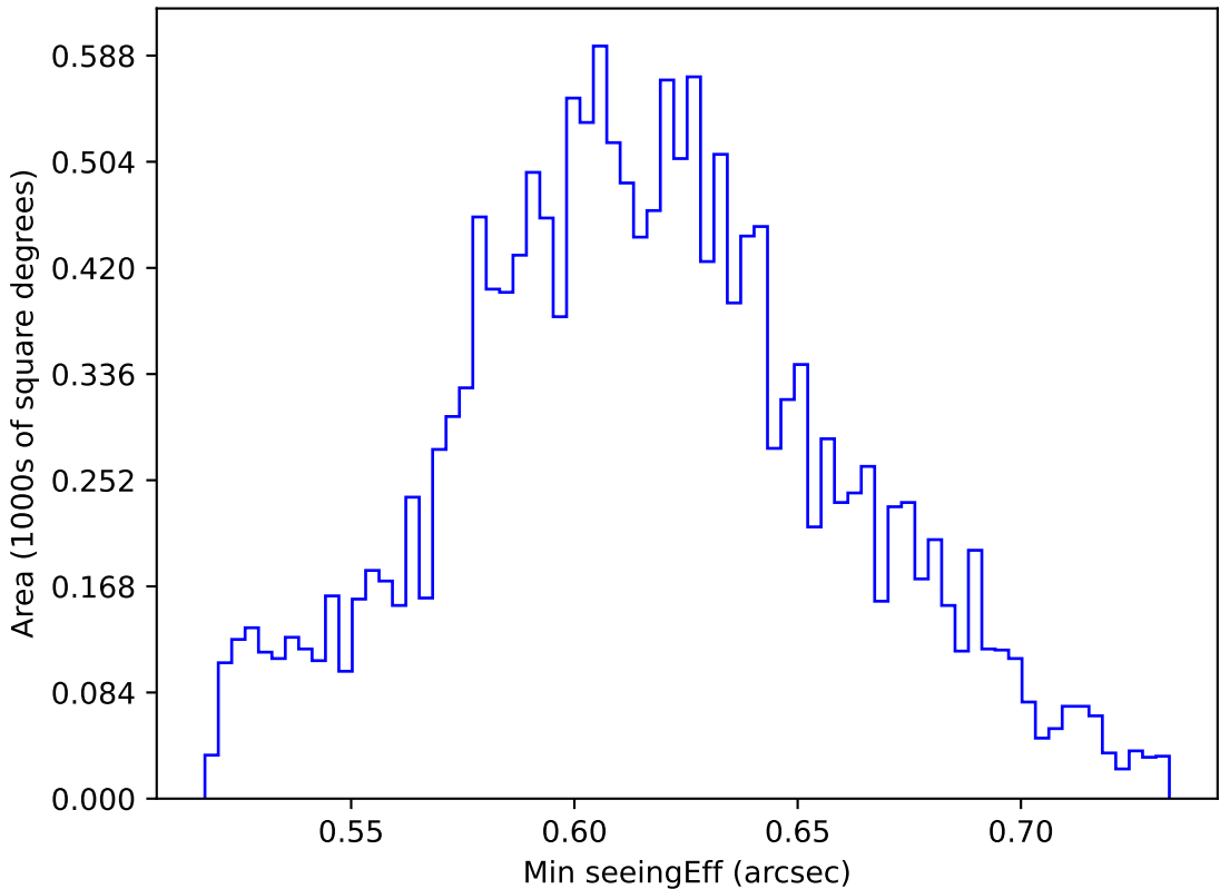
too_elab_r64_d3_griz_v3.4_10yrs WFD z band: Min seeingEff
