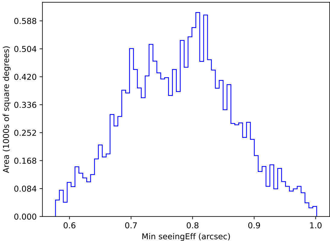
too_elab_r64_d3_griz_v3.4_10yrs WFD u band: Min seeingEff
