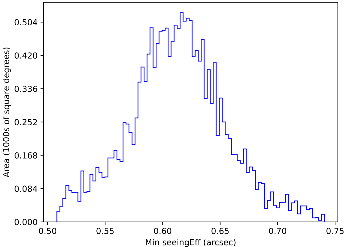
too_elab_r64_d3_griz_v3.4_10yrs WFD r band: Min seeingEff
