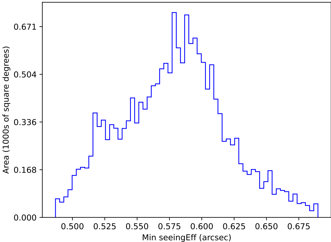
too_elab_r64_d3_griz_v3.4_10yrs WFD all bands: Min seeingEff
