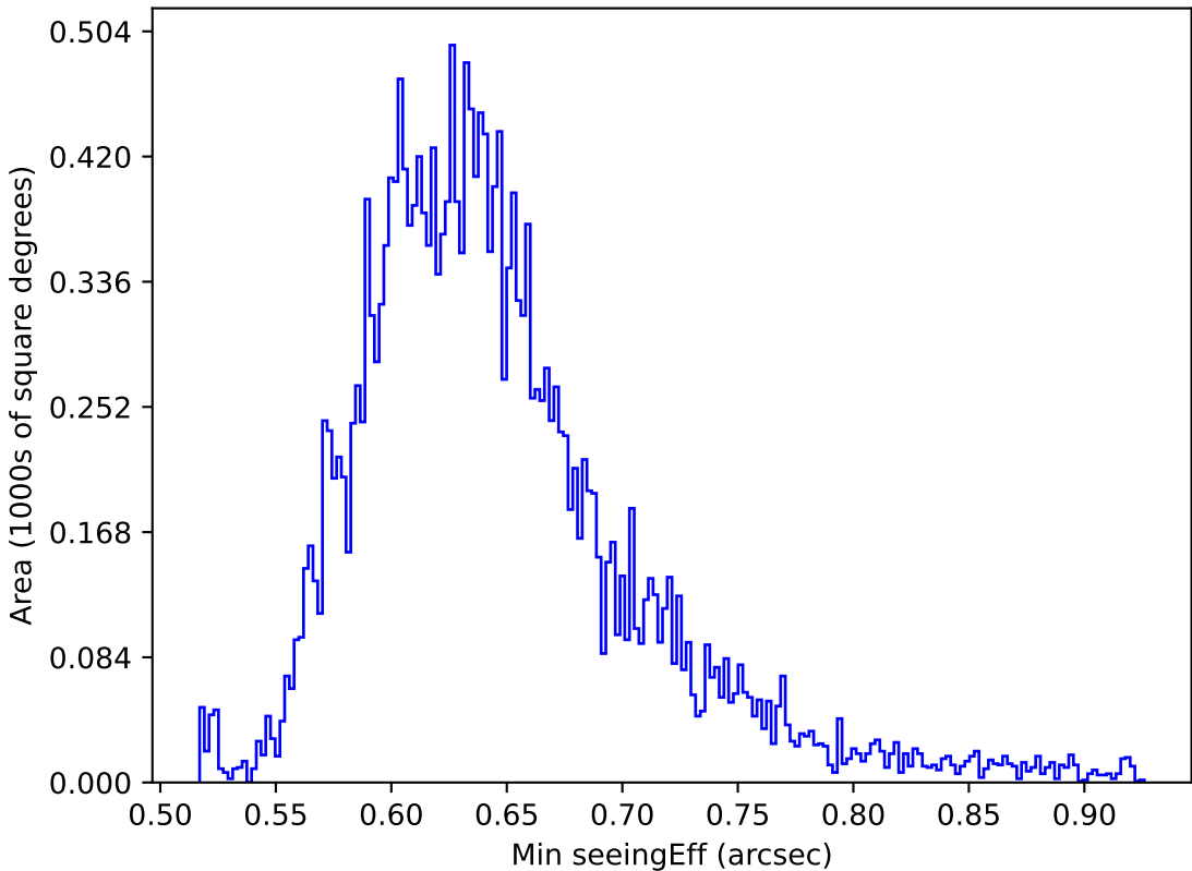
too_elab_r64_d3_griz_v3.4_10yrs All sky y band: Min seeingEff
