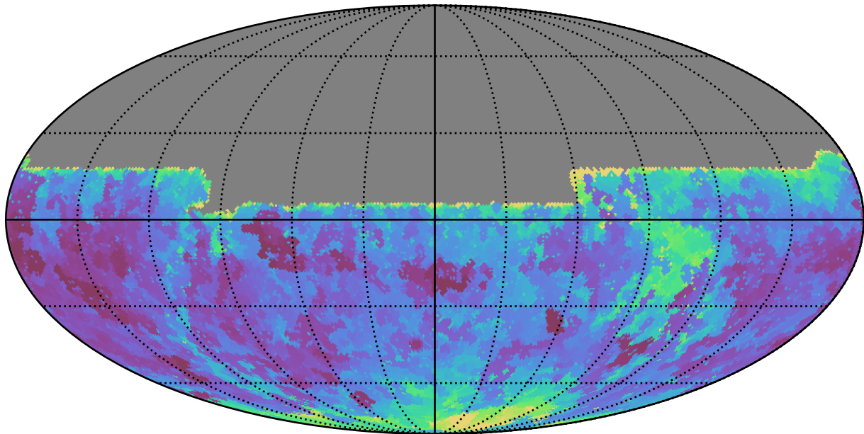
too_elab_r64_d3_griz_v3.4_10yrs All sky u band: Min seeingEff
