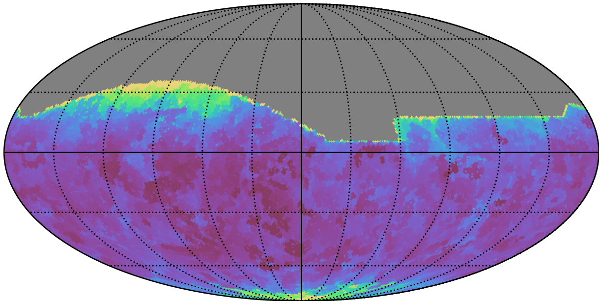
too_elab_r64_d3_griz_v3.4_10yrs All sky r band: Min seeingEff
